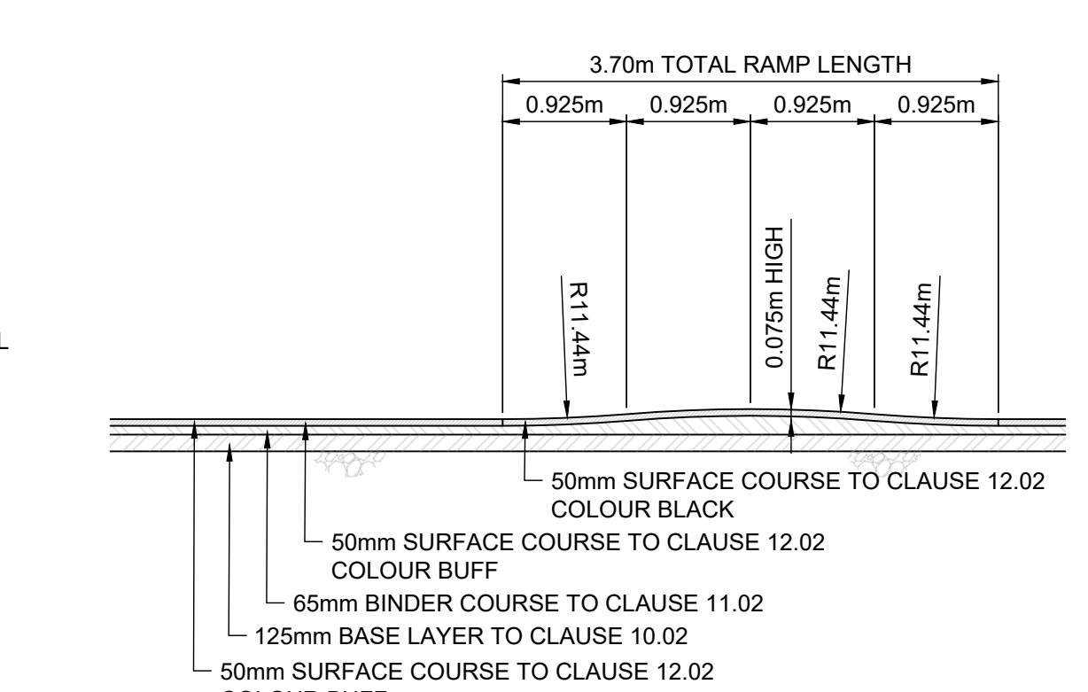
75mm HIGH SINUSOIDAL RAMP & SURFACING
