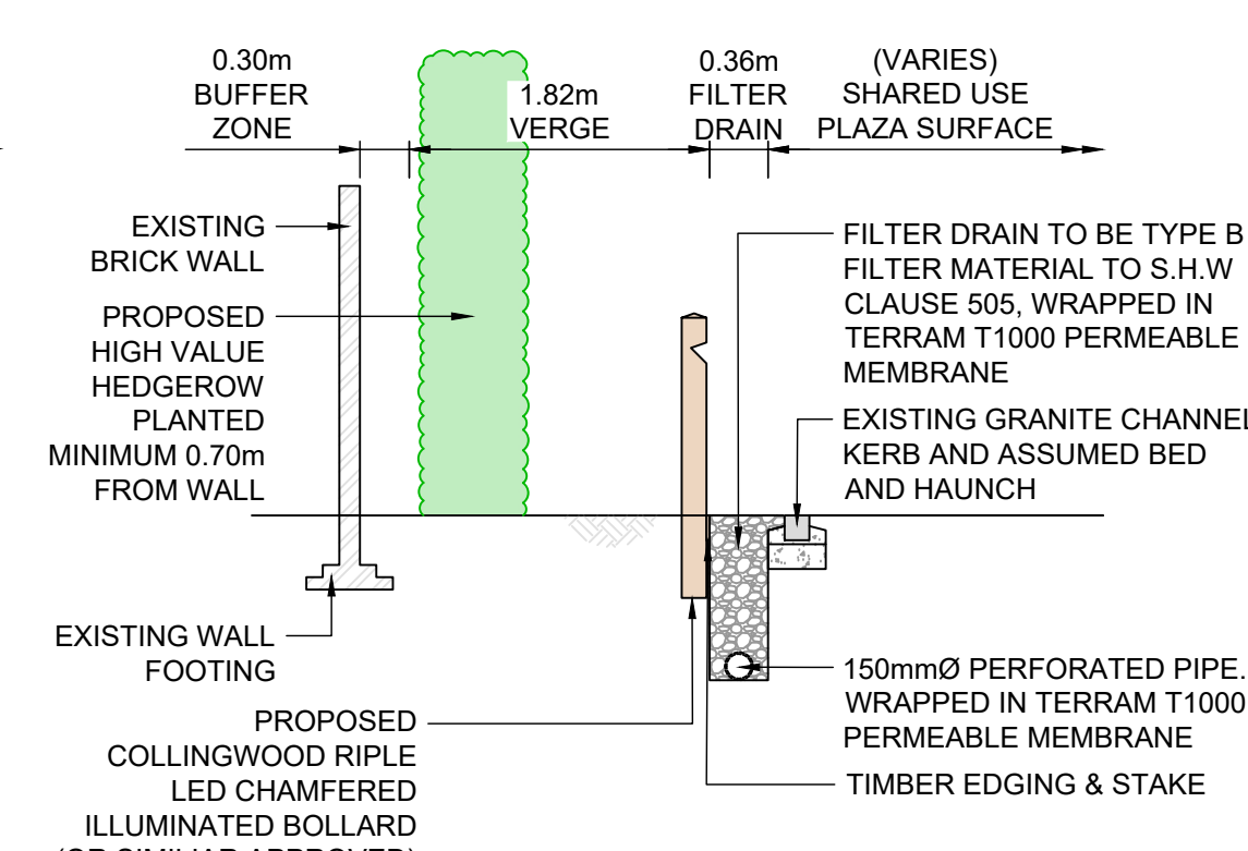
SECTION B-B
